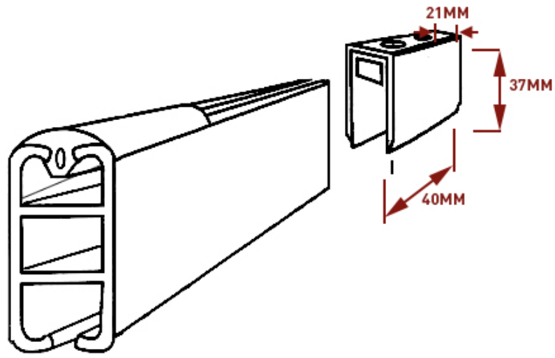
DETAIL OF WALL SUPPORT BRACKET
